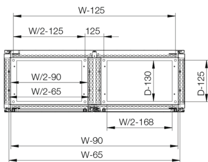
Sectional top view (without bottom plates)
