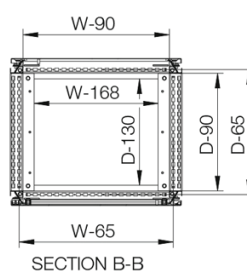
Sectional top view (without bottom plates)
