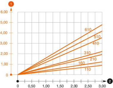
Belastingsdiagram console AW 30
