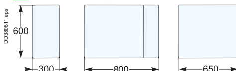
Switchboard 2 - combination of IP30 cubicles with transparent doors.
