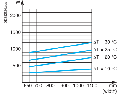
IP3X cubicle, 400 mm deep
