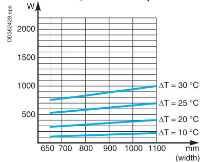
IP55 cubicle, 400 mm deep
