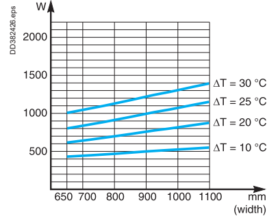
IP3X cubicle, 800 mm deep
