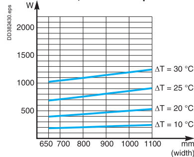
IP55 cubicle, 800 mm deep
