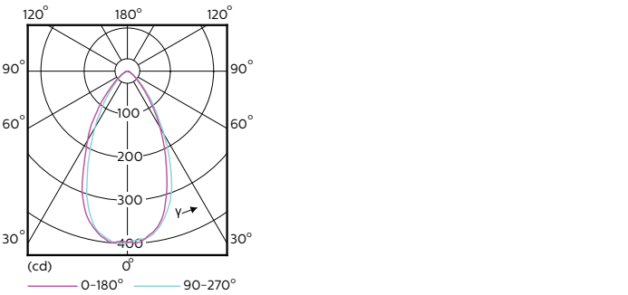
Light Distribution Diagram - MAS LED spot VLE D 4.9-50W GU10 927 60D
