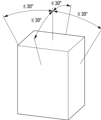
Figure 41: Installation position
