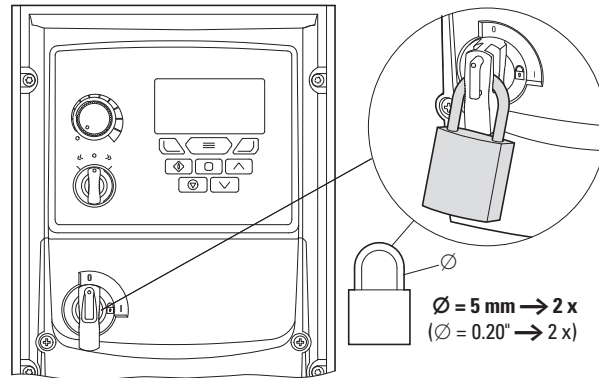
Figure 52: DA1-...-A6SO with padlock
