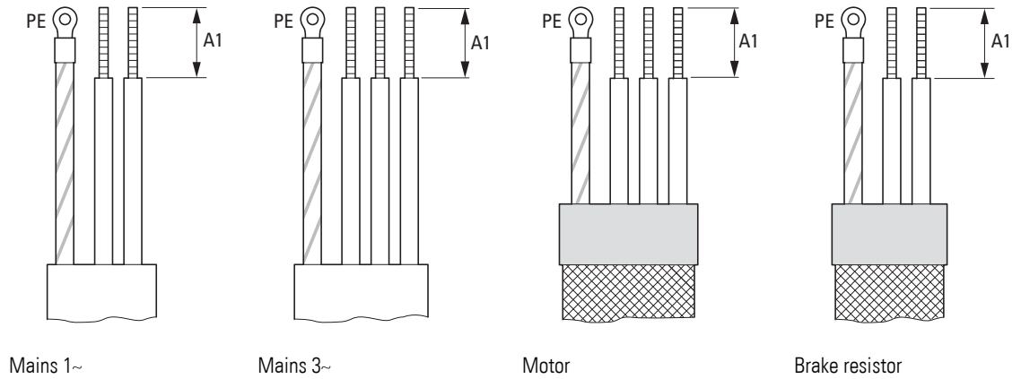
Figure 67: Connection cables
