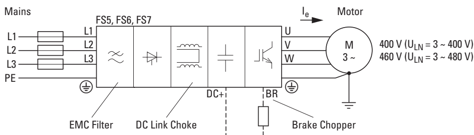
Figure 16: DA1-34...FB-... with DC link choke
