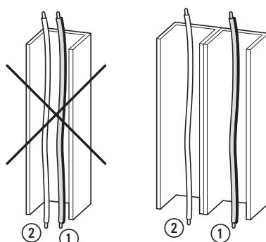
Figure 54: Separate routing
