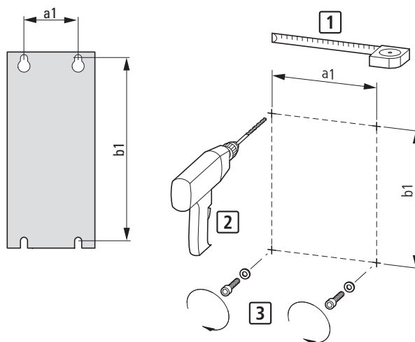
Figure 45: Mounting dimensions
