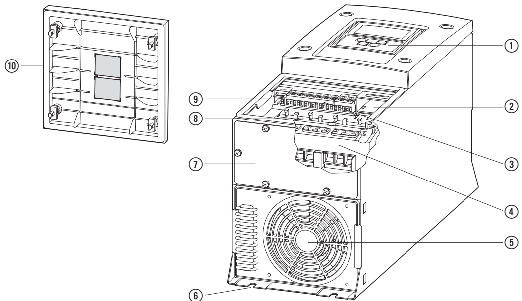
Figure 9: DA1 designations (here: FS4, IP55)
