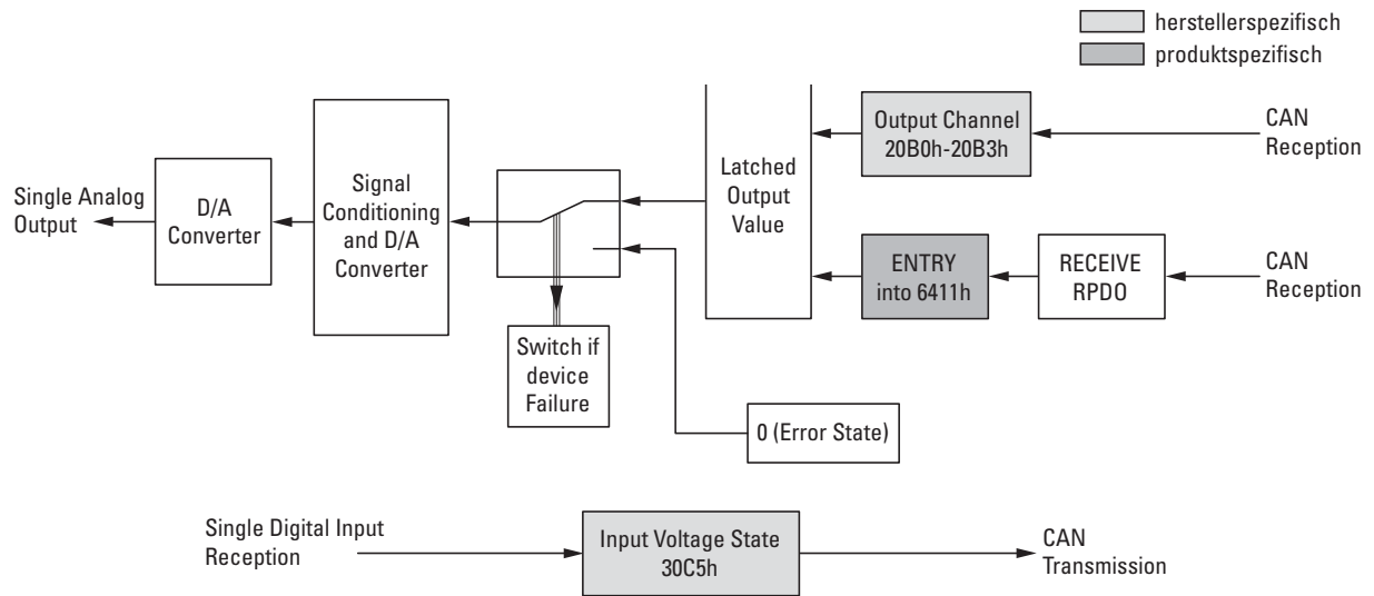
Figure 88: Block diagram showing the various CANopen objects for analog outputs
