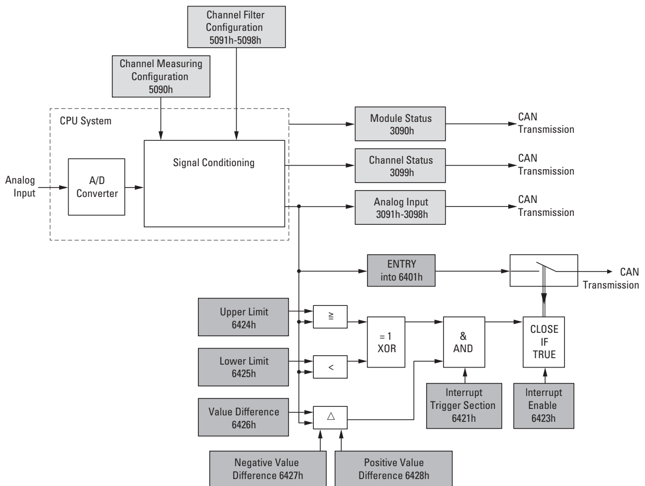
Figure 76: Block diagram showing the various CANopen objects for analog inputs
