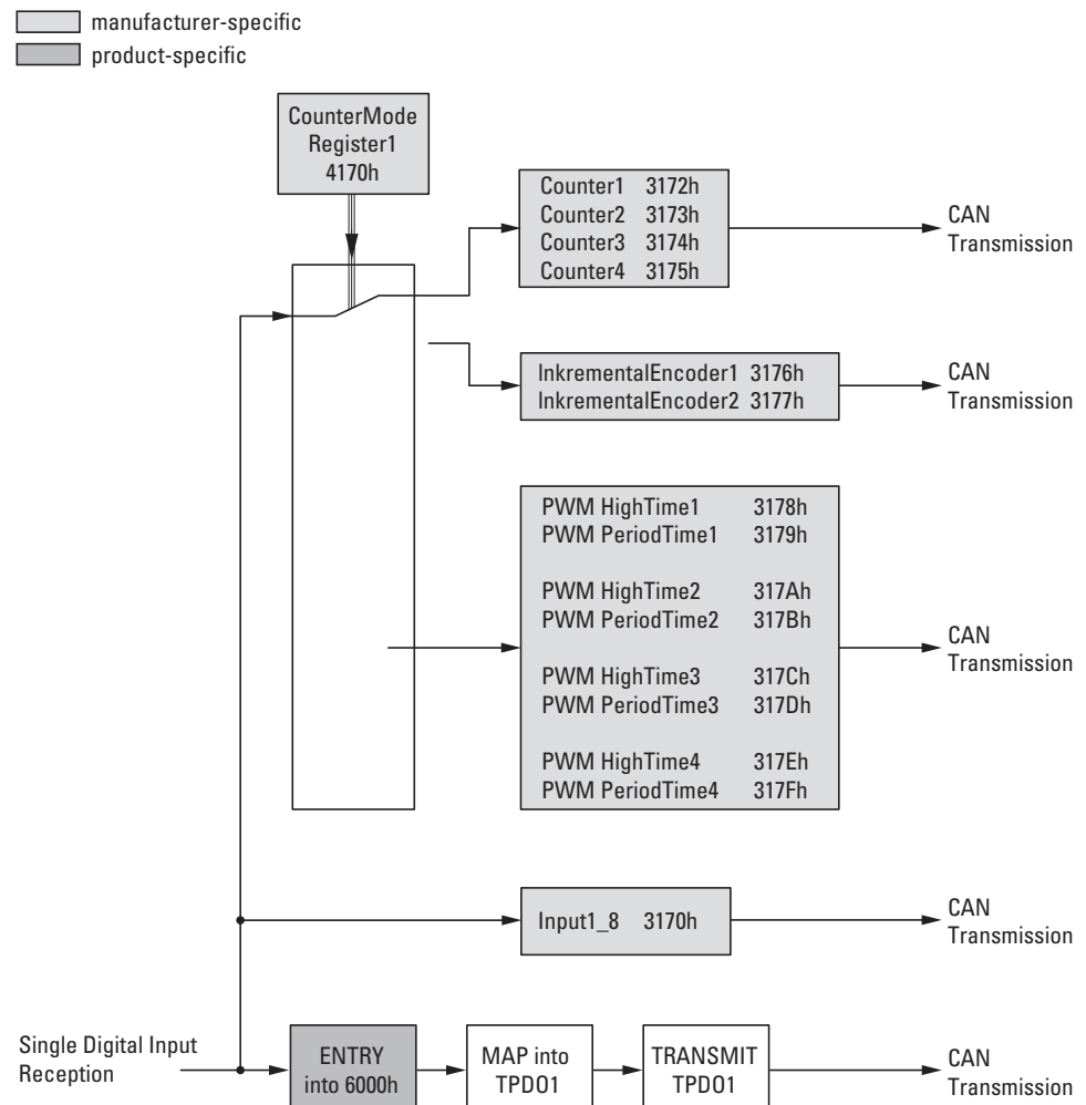
Figure 68: Block diagram showing the various CANopen objects for digital inputs
