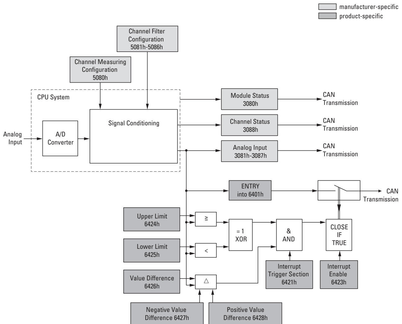
Figure 75: Block diagram showing the various CANopen objects for analog inputs
