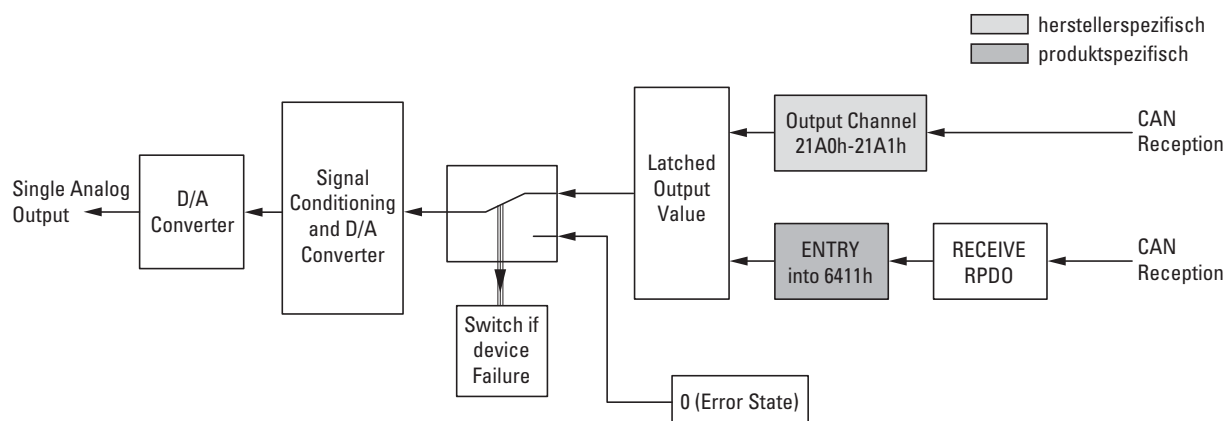
Figure 82: Block diagram showing the various CANopen objects for analog outputs
