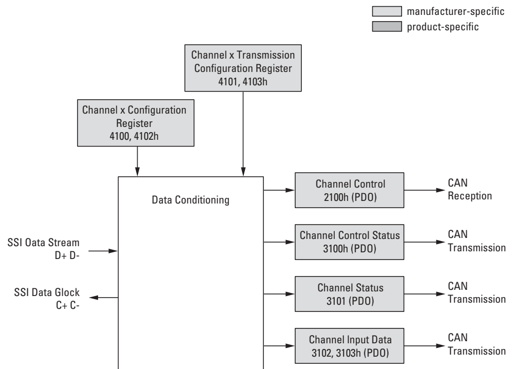
Figure 94: Block diagram showing the various CANopen objects for transmitting data streams
