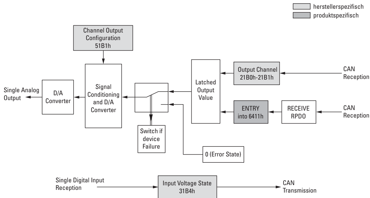
Figure 86: Block diagram showing the various CANopen objects for analog outputs
