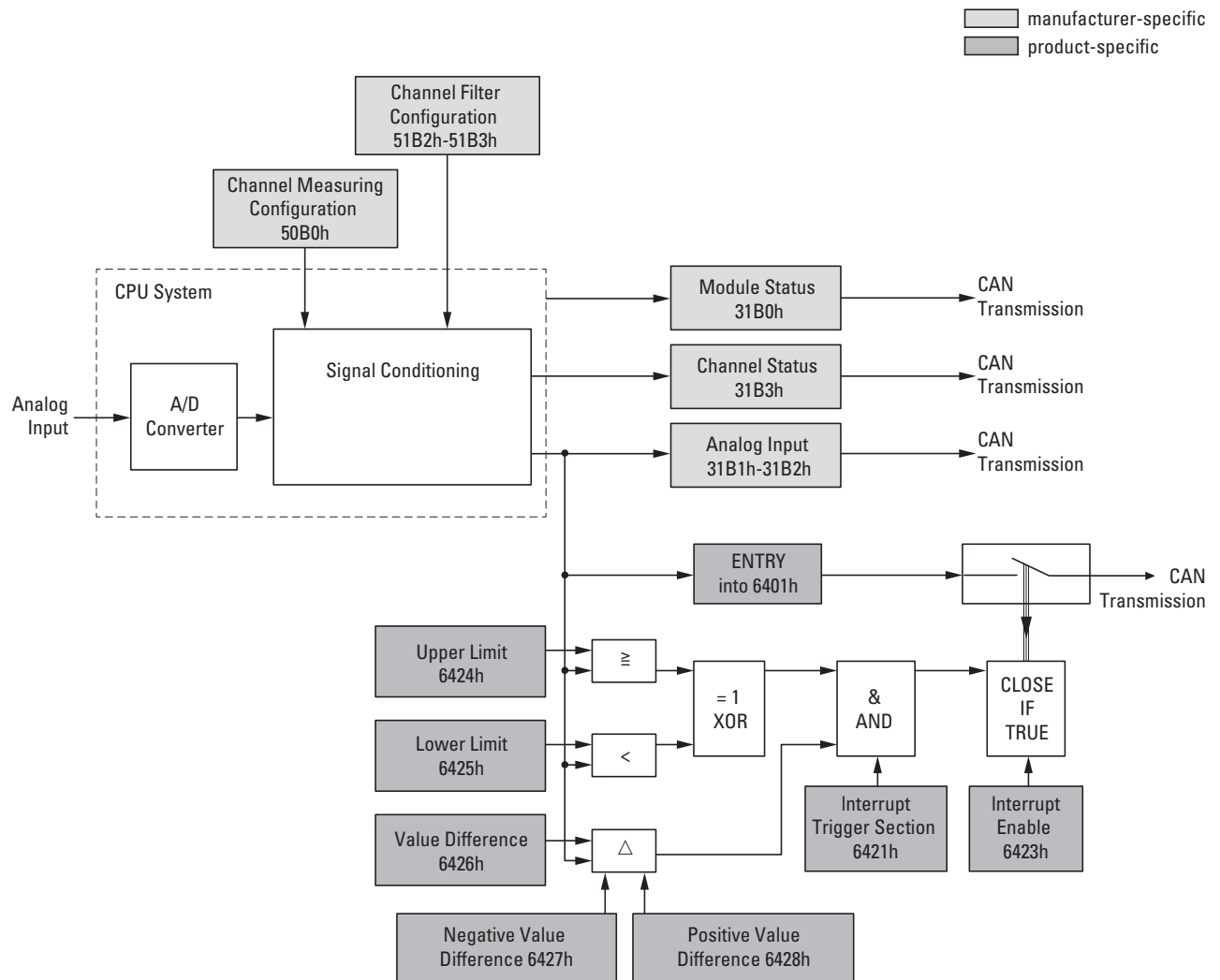
Figure 85: Block diagram showing the various CANopen objects for analog inputs
