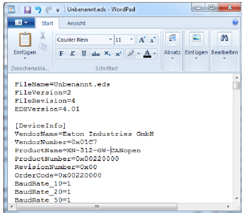
Figure 30: Header of an EDS file for XN-312-GW-CAN
