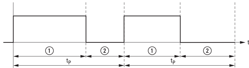
Figure 71: PWM signal measurement
