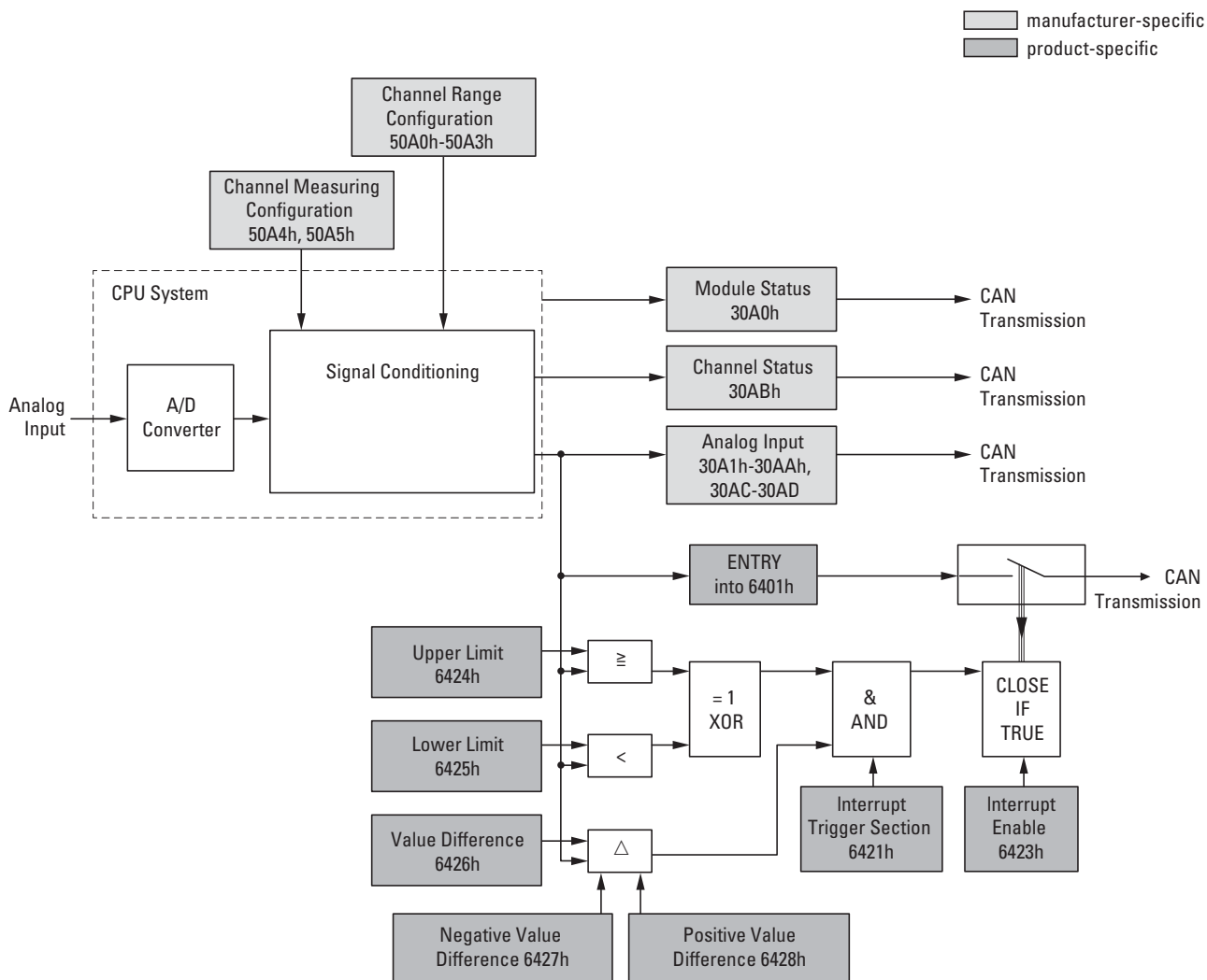
Figure 78: Block diagram showing the various CANopen objects
