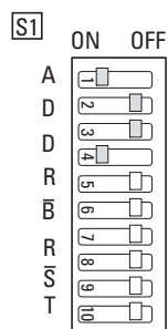
Figure 8: Example: Setting field bus address 18_{\text{dec}} on the gateway
