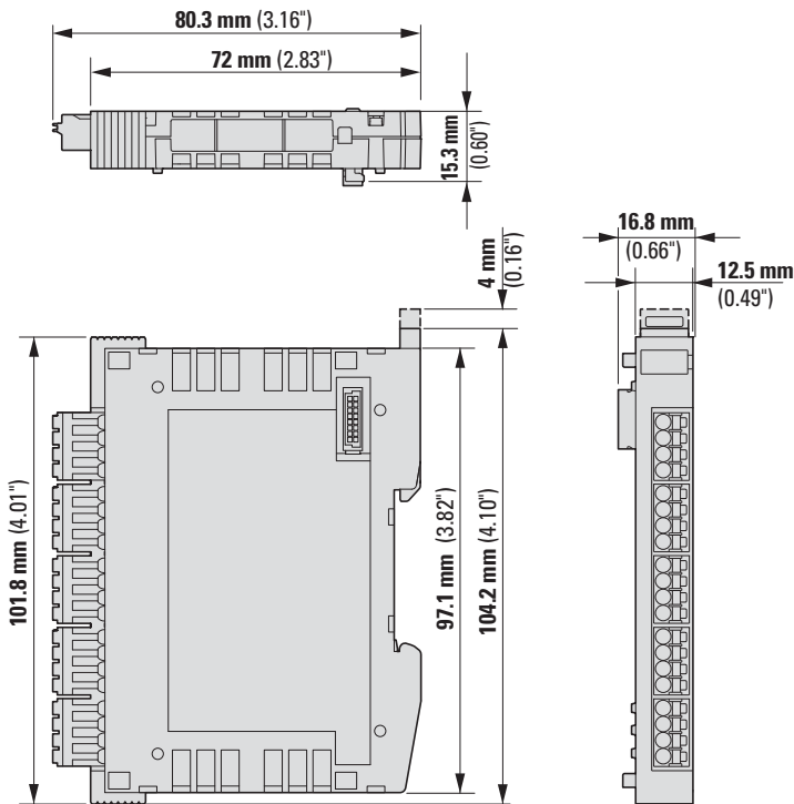
Figure 103: Dimensions XN-312-GW-CAN
