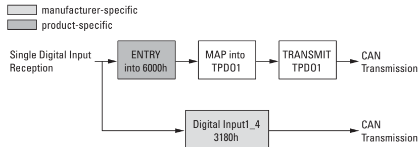
Figure 64: Block diagram showing the various CANopen objects for digital inputs
