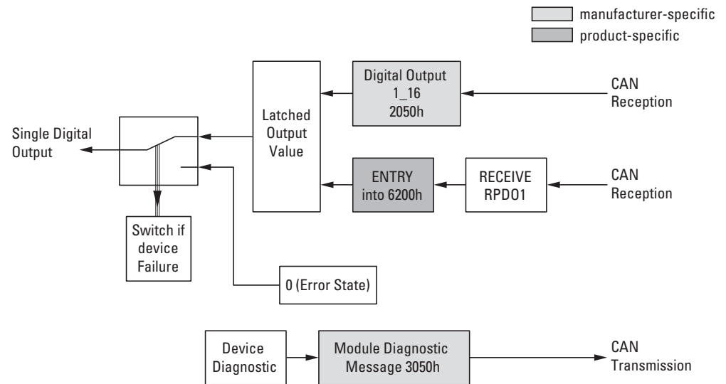
Figure 63: Block diagram showing the various CANopen objects for digital outputs
