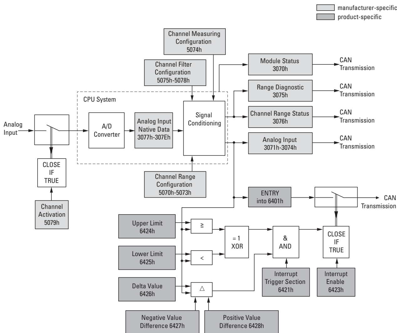
Figure 74: Block diagram showing the various CANopen objects for analog inputs
