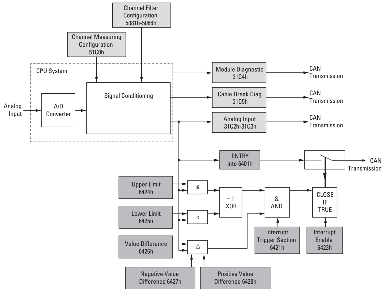
Figure 73: Block diagram showing the various CANopen objects for transmitting datastreams
