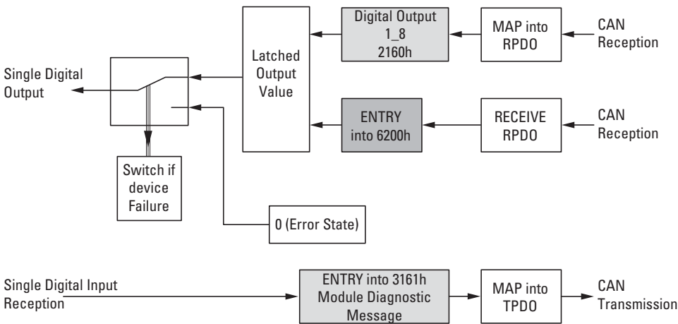
Figure 67: Block diagram showing the various CANopen objects for digital outputs
