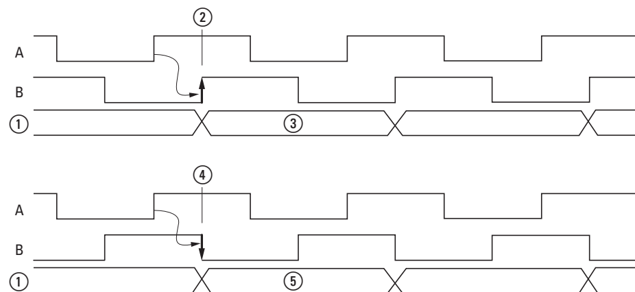
Figure 92: Signal diagram for signals A and B
