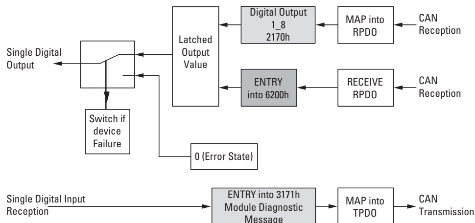
Figure 69: Block diagram showing the various CANopen objects for digital outputs
