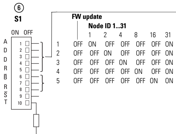
Figure 5: DIP switches for setting the gateway's node ID
