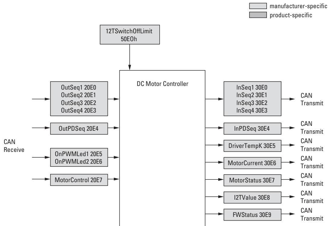
Figure 90: Block diagram showing the various CANopen objects
