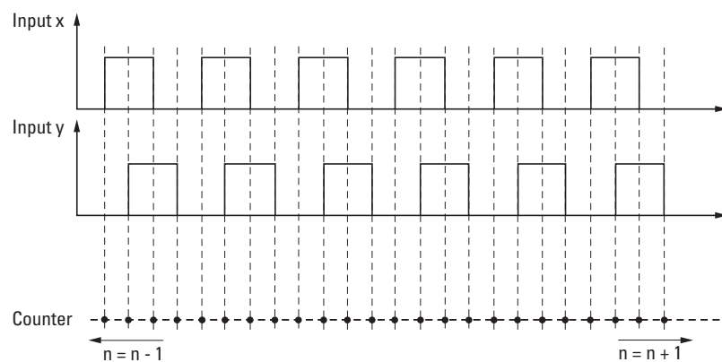
Figure 70: Timing diagram showing how inputs (x/y) = (1/2) or (3/4) of the incremental encoder register in the XN-322-16DIO-PC05 module count with X4 encoding
