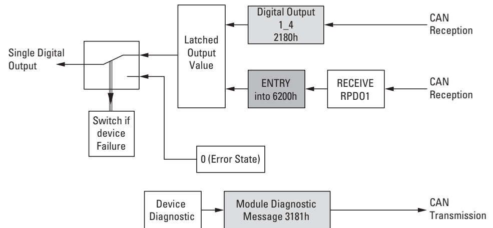
Figure 65: Block diagram showing the various CANopen objects for digital outputs
