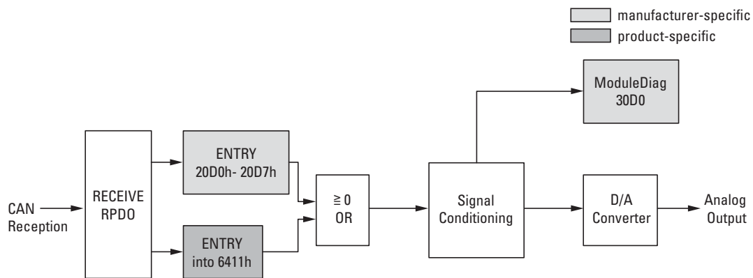
Figure 80: Block diagram showing the various CANopen objects for analog outputs
