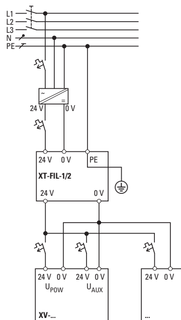
Figure 26: Engineering example for integration of radio interference suppression filters
