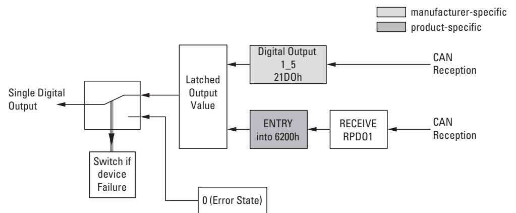
Figure 60: Block diagram showing the various CANopen objects for transmitting data streams
