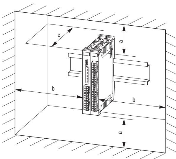
Figure 10: Horizontal installation only!
