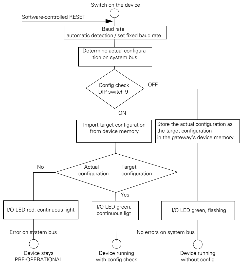
Figure 28: Switching on the device with and without a config check
