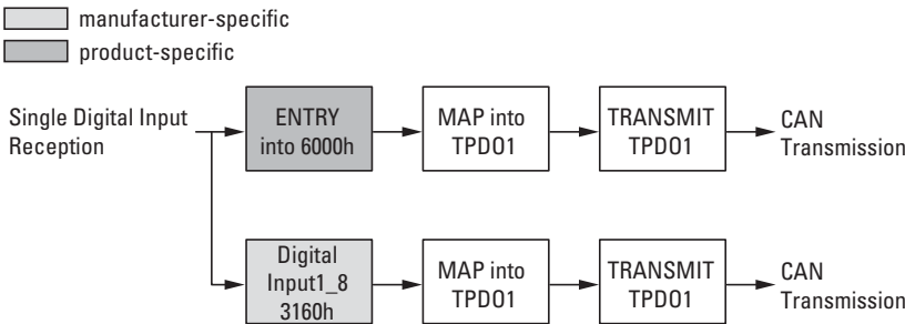
Figure 66: Block diagram showing the various CANopen objects for digital inputs
