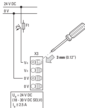
Figure 21: Connection of power supply
