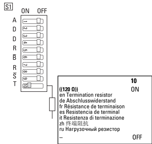
Figure 9: Activated bus termination resistor
