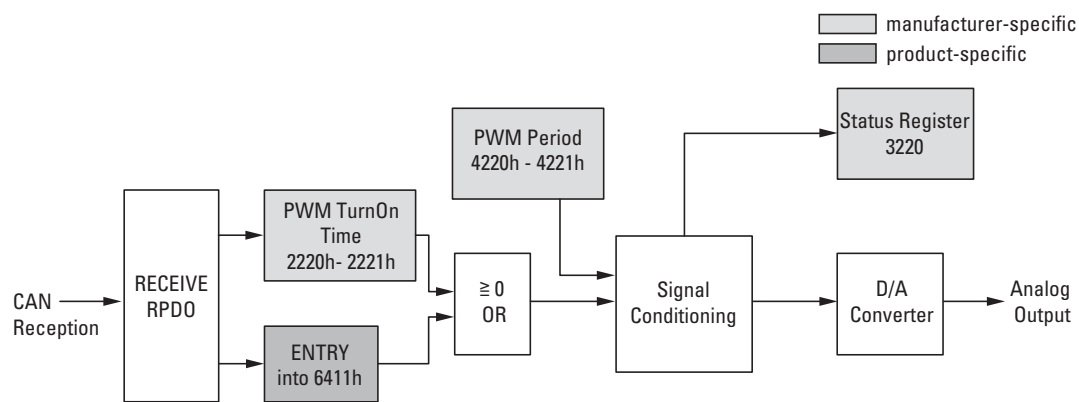
Figure 95: Block diagram showing the various CANopen objects for transmitting data streams
