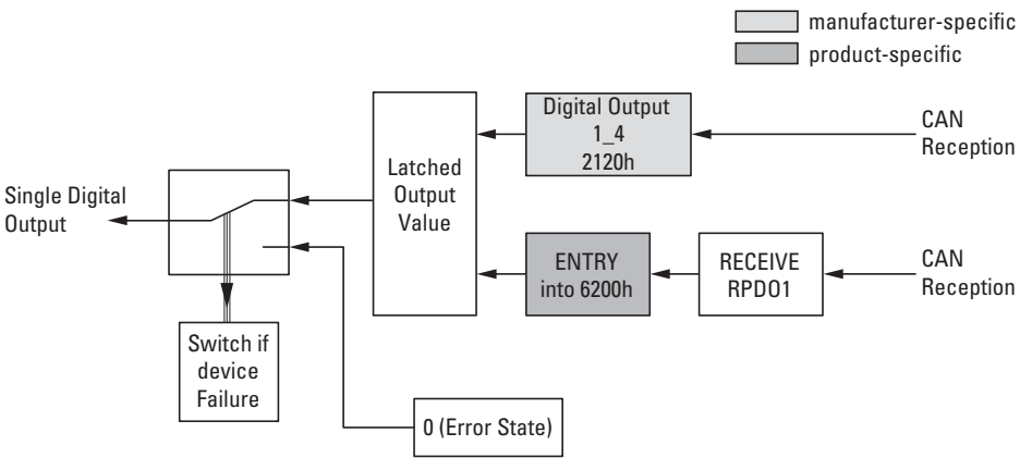
Figure 59: Block diagram showing the various CANopen objects for digital outputs
