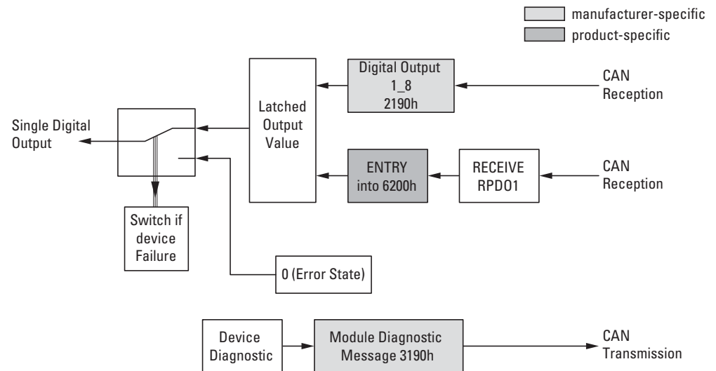
Figure 61: Block diagram showing the various CANopen objects for digital outputs
