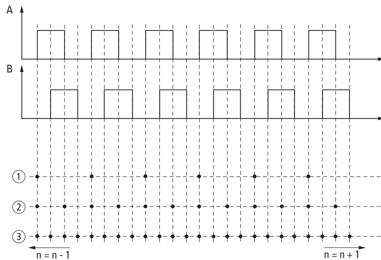
Figure 93: Signal diagram
