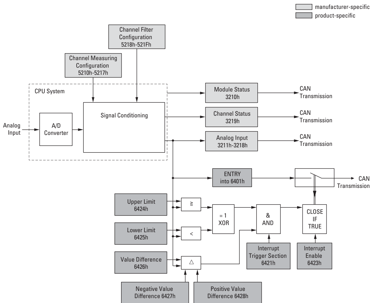
Figure 77: Block diagram showing the various CANopen objects for transmitting data streams
