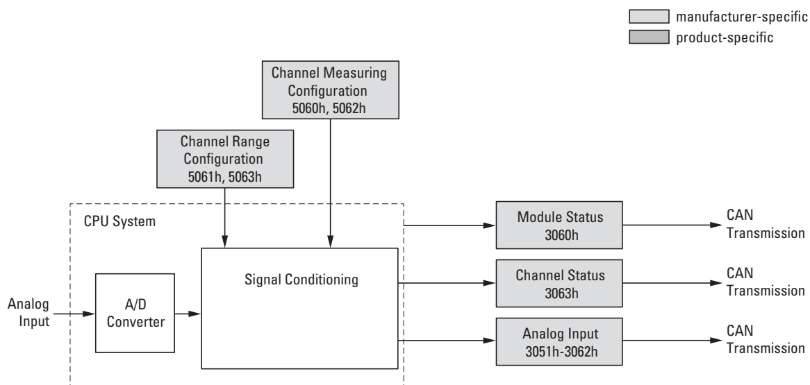
Figure 89: Block diagram showing the various CANopen objects
