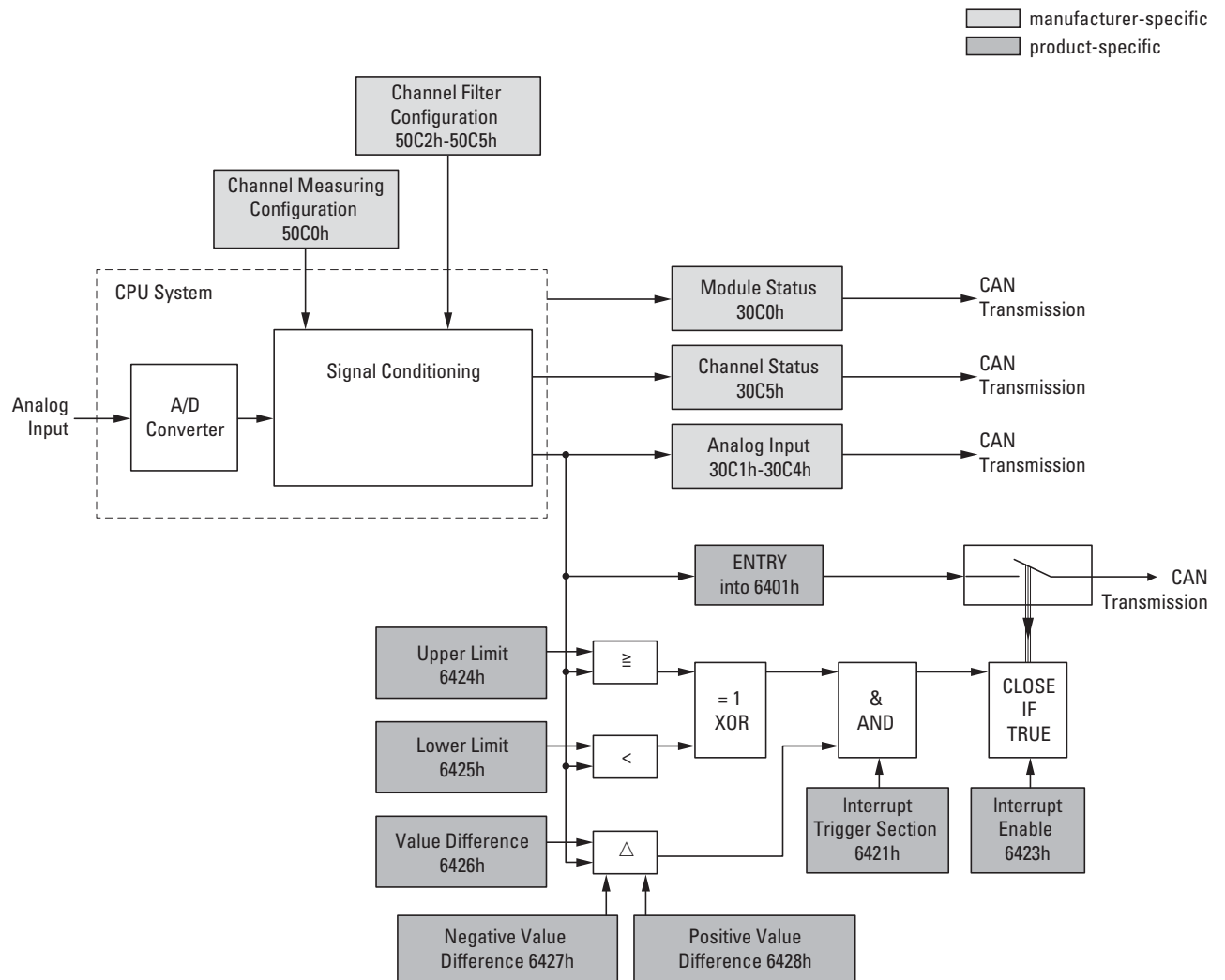
Figure 87: Block diagram showing the various CANopen objects for analog inputs
