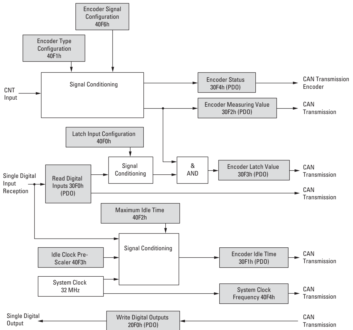
Figure 91: Block diagram showing the various CANopen objects for analog inputs
