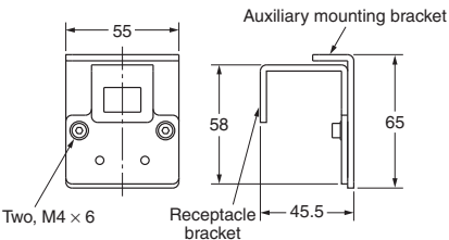
Auxiliary Mounting Bracket and Receptacle Bracket
