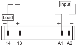
Terminal Arrangement/ Internal Connection Diagram (TOP VIEW)
