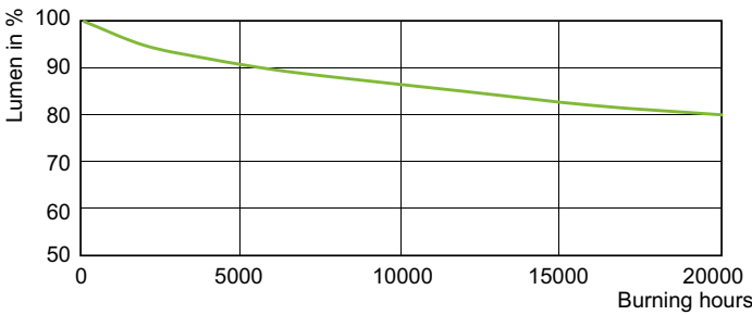
Lumen Maintenance Diagram - MASTER CityWh CDO-TT Plus 100W/828 E40
