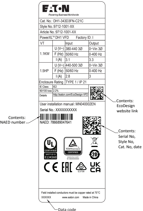
Figure 3. Rating label—DH1
