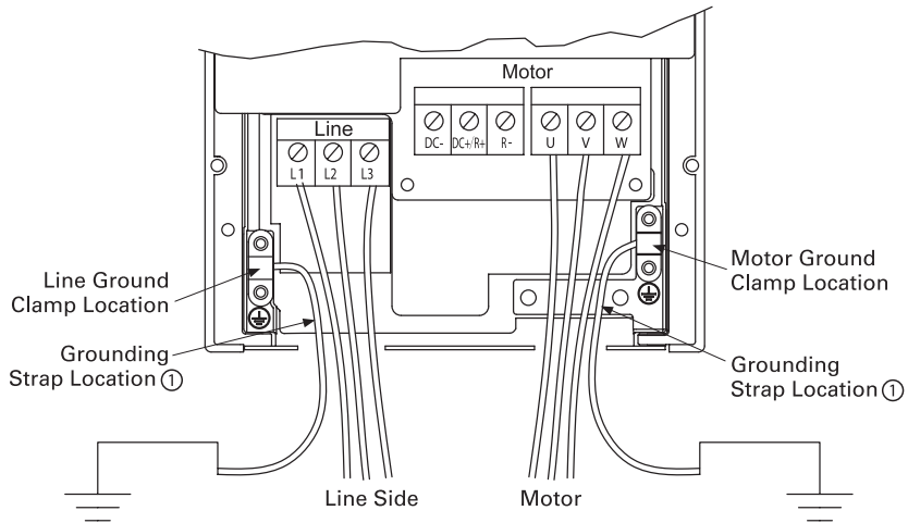
Figure 24. Ground wiring
