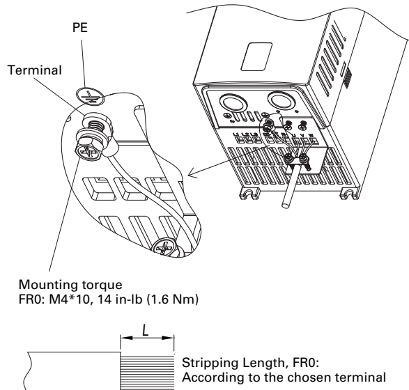
Figure 30. FR0 grounding
