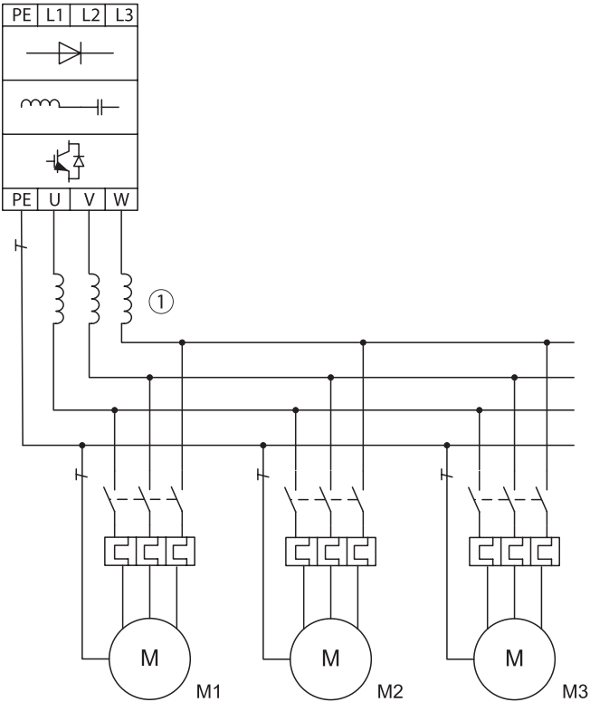
Figure 14. Parallel connection
