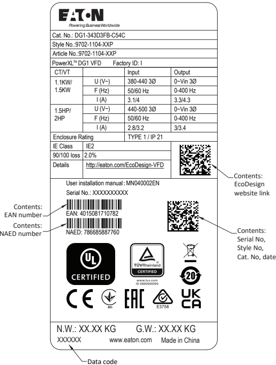
Figure 4. Carton label—DG1
