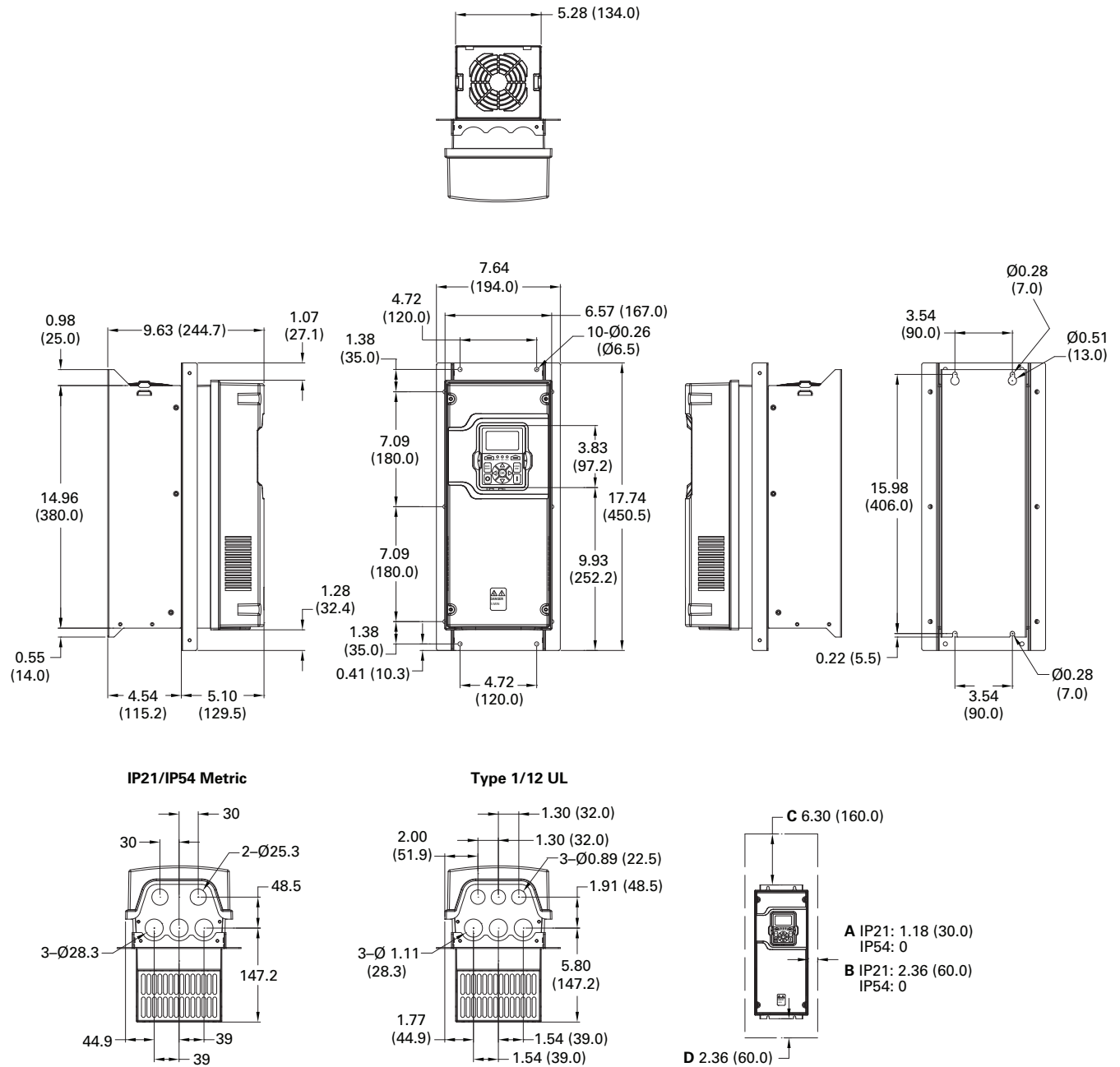
Figure 44. FR2 dimension drawing flange mount
