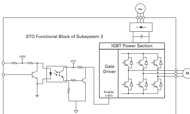
Figure 53. Functional block diagram
