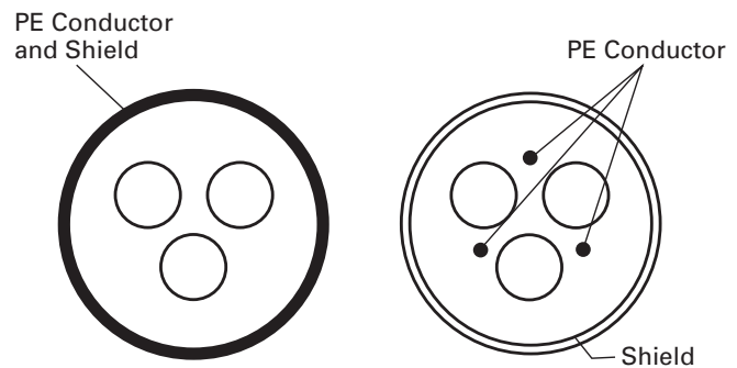
Figure 35. Cable description
