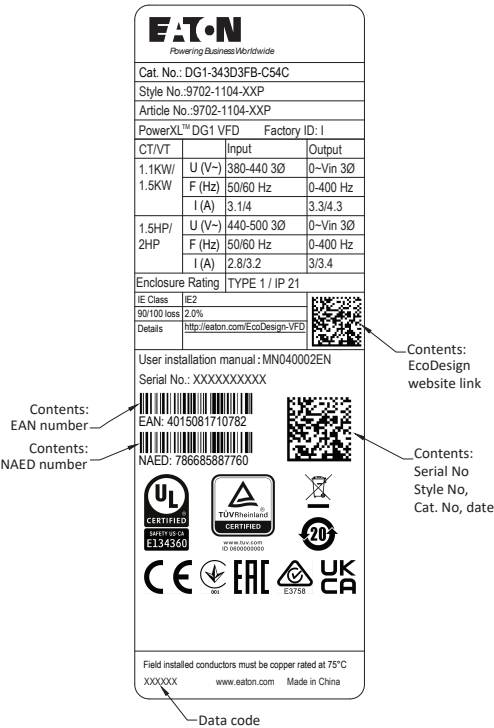
Figure 2. Rating label—DG1
