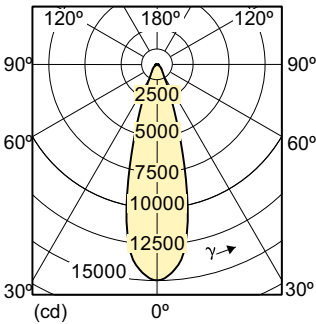
Light Distribution Diagram - MC CDM-R Elite 70W/930 E27 PAR30L 30D
