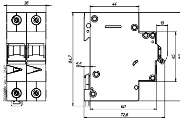
1+N-poles
