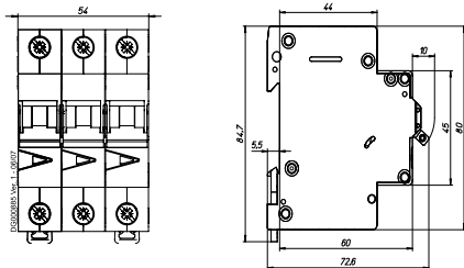
3-poles
