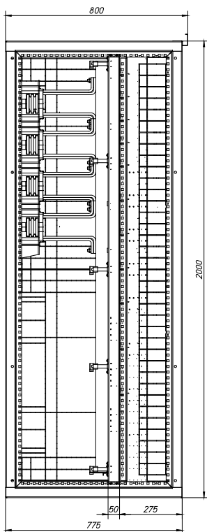
XF_NZM1_3_F4_800_S_mMS
