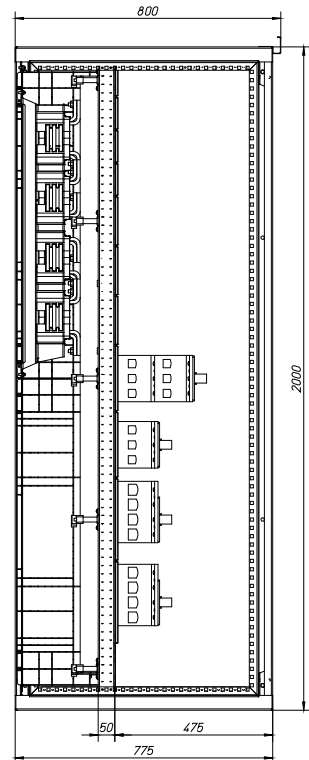
XF_NZM1_3_F2b_800_S
