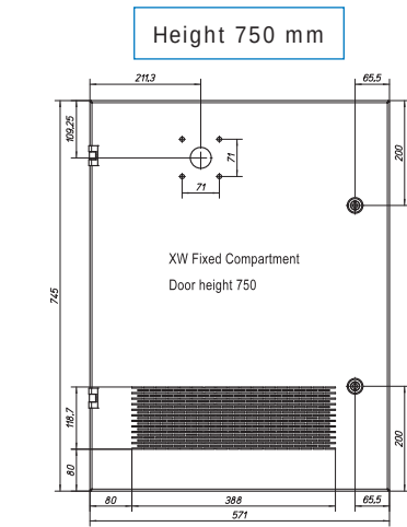
MCC_Fix_H600_H750_Door
