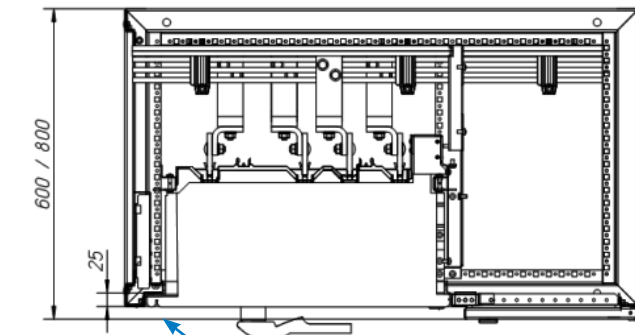
Installation of PIFT modules
