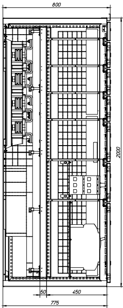
XF_NZM1_3_F4_800_S_oMS_BS_350
