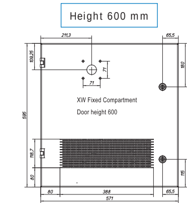
MCC_Fix_H600_H750_Door
