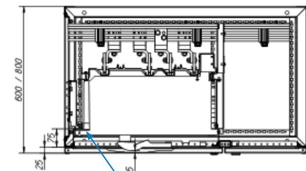
Installation of PIFT modules
