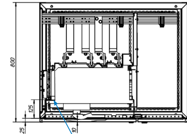
Installation of PIFT modules
