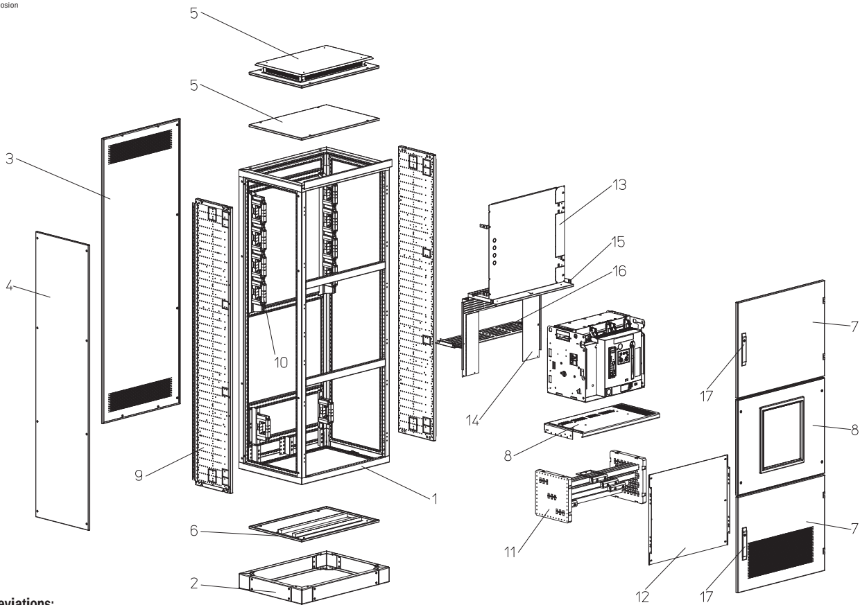
IZM_Explosion
