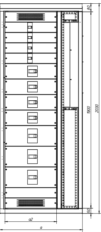
XF_NZM1_3_F4_600_V_oFP
