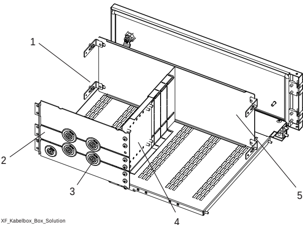
XF_Kabelbox_Box_Solution
