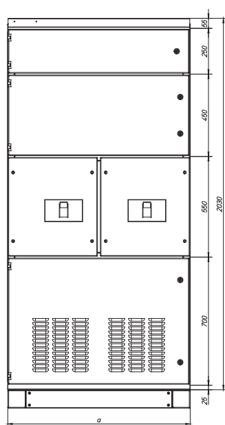
2xNZM4_SbS
