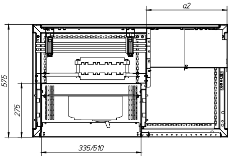
XF_NZM1_3_F4_600_D_BS
