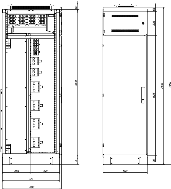
XF_2b_Katalog_1_W600
