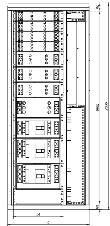
XF_NZM1_3_F2b_800_V
