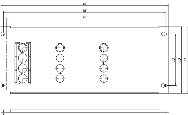
BS_mounting plates_V1
