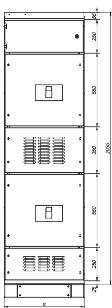
Stacked-NZM4
