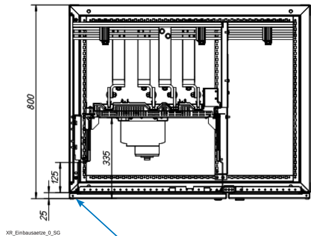
Installation of switchgear modules
