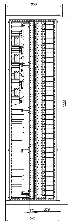
XF_NZM1_3_F4_600_S_mMS
