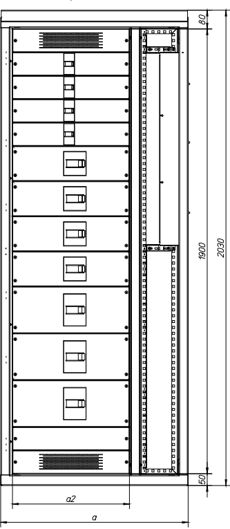
XF_NZM1_3_F4_800_V_mFP_350
