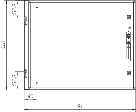
Door to switchgear area - height 640 mm (1/3 door)
