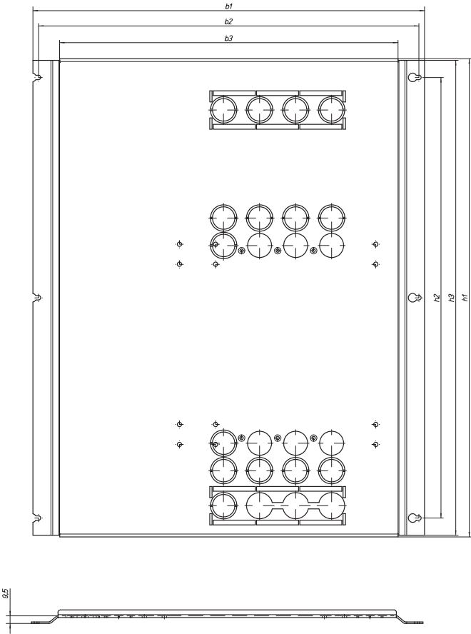
BS_mounting plates_V2
