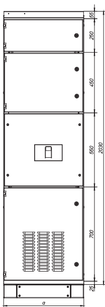
Single-NZM4
