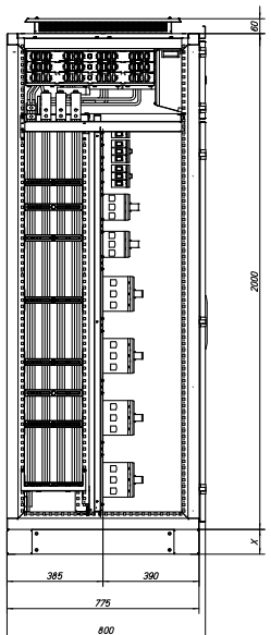
XF_2b_W1000
