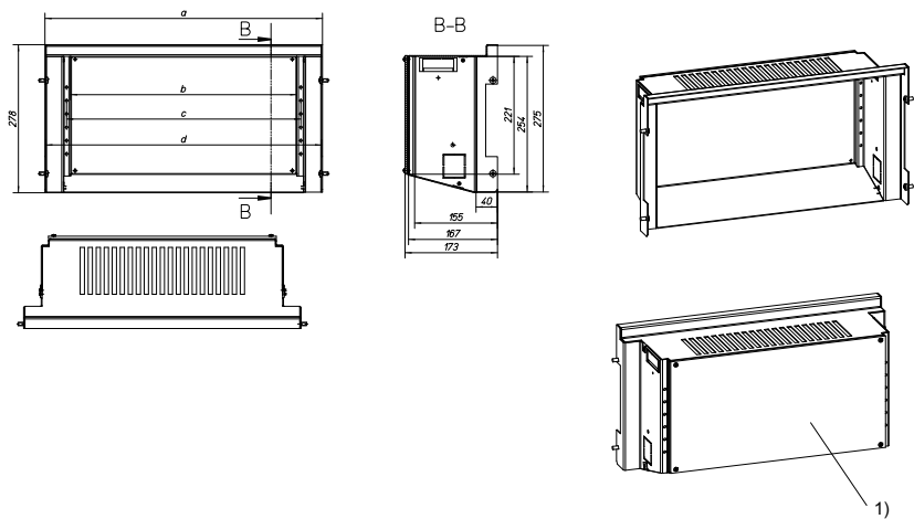
1) Additional insulating partition at the rear
