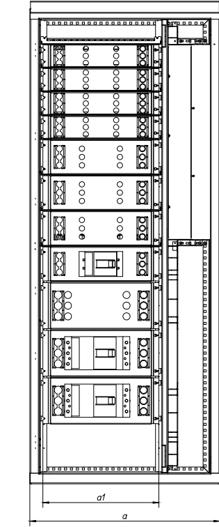
XF_NZM1_3_F4_800_V_oFP_350
