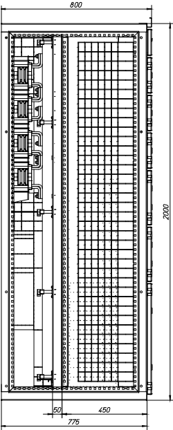
XF_NZM1_3_F4_800_S_mMS_BS_350
