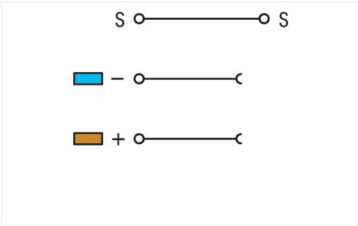
270-560 Sensor terminal block, 270 Series, CAGE CLAMP®
