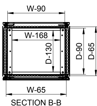
Sectional top view (without bottom plates)
