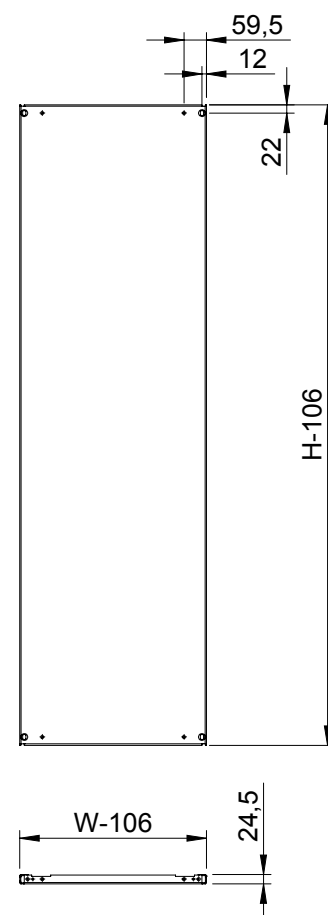
Mounting plate
