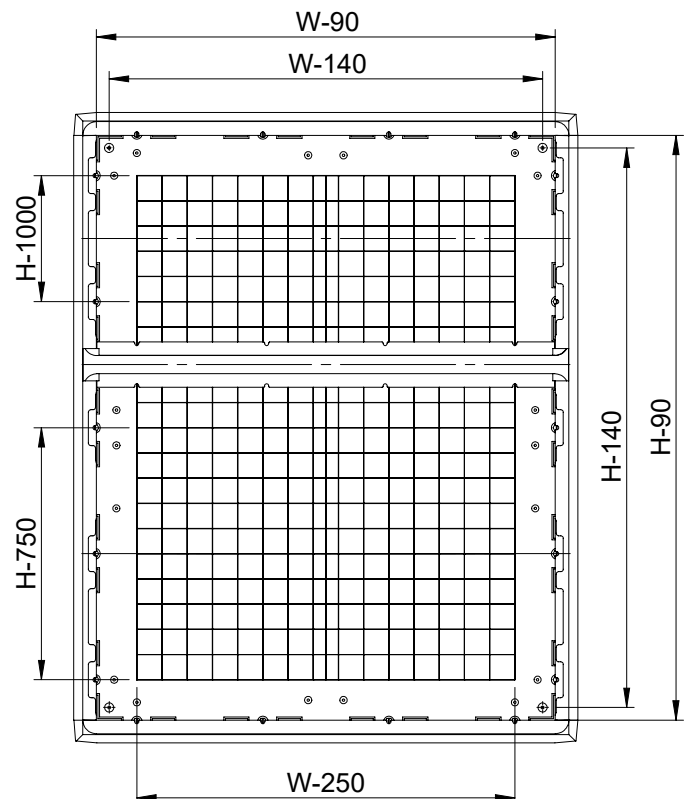
Front view H=1250 (without doors)
