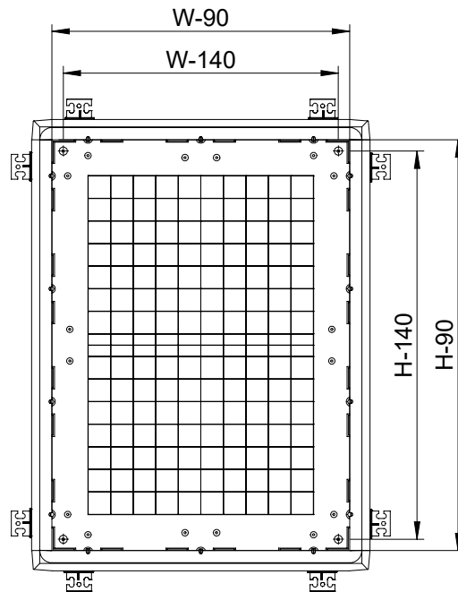
Front view (without door)
