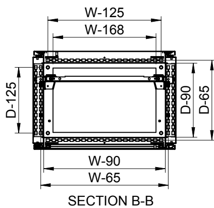
Sectional top view (without bottom plates)
