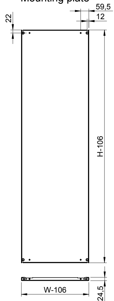
Mounting plate
