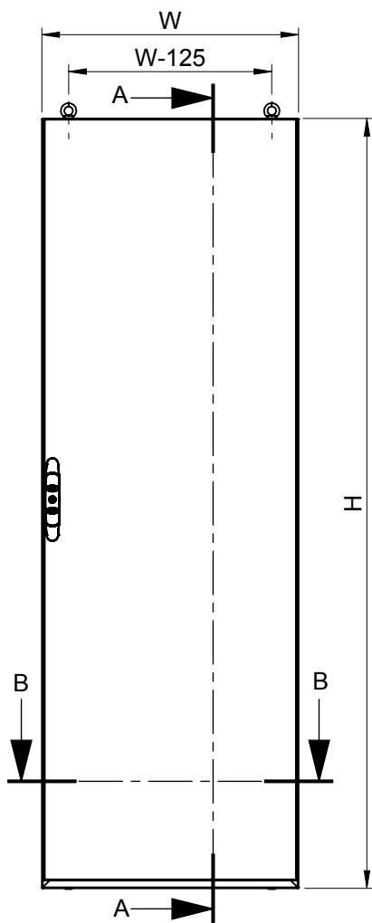
Front view
