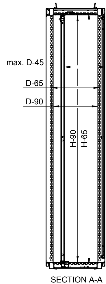
Mounting plate
