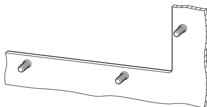
Fig. 18: M4 x 12 weld studs on sheet
