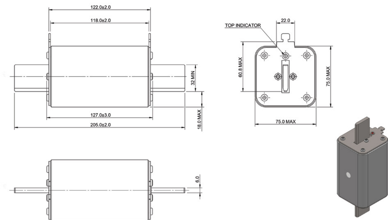
Dimensions (mm) - Size 3L Bladed with and without top indicator
