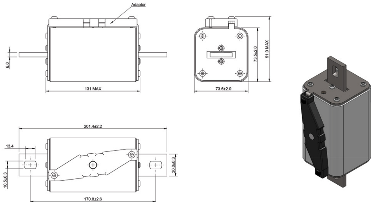
Dimensions (mm) - size 3 Bolted
