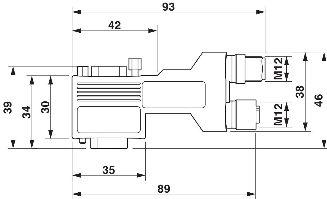
Maatschets SUBCON-PLUS...90X...M12, lange 90°-variant
