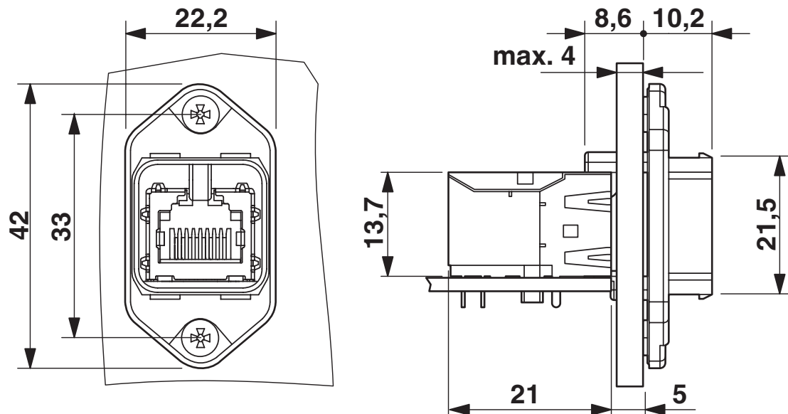
Push-pull-aanbouwraam, RJ45
