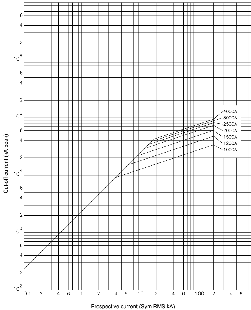
Cut-off curve - 1000 A to 4000 A
