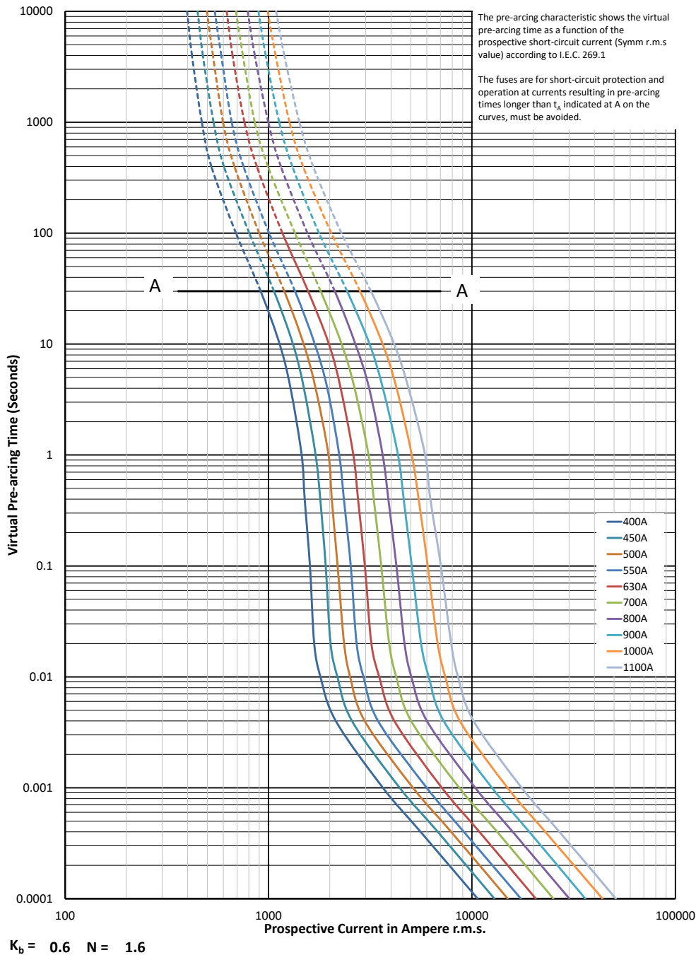
Time-current curve - Size 2, 400 A to 1100 A
