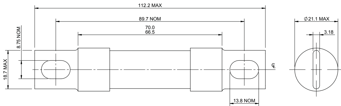
Dimensions (in) - 35 A to 60 A
