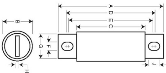
Dimensions (in) - 70 A to 600 A
