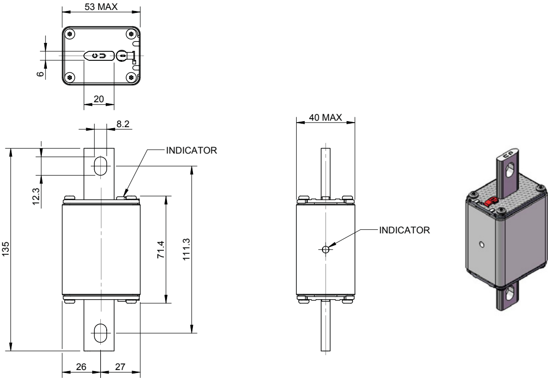
Dimensions (mm) NH1 Blade with bolt holes
