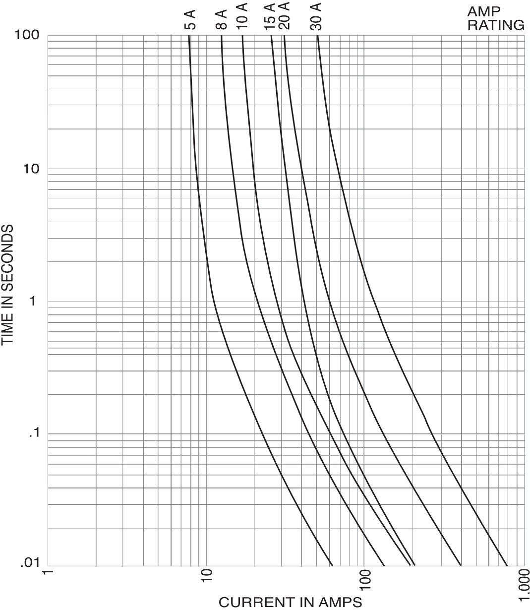
Time current curve
