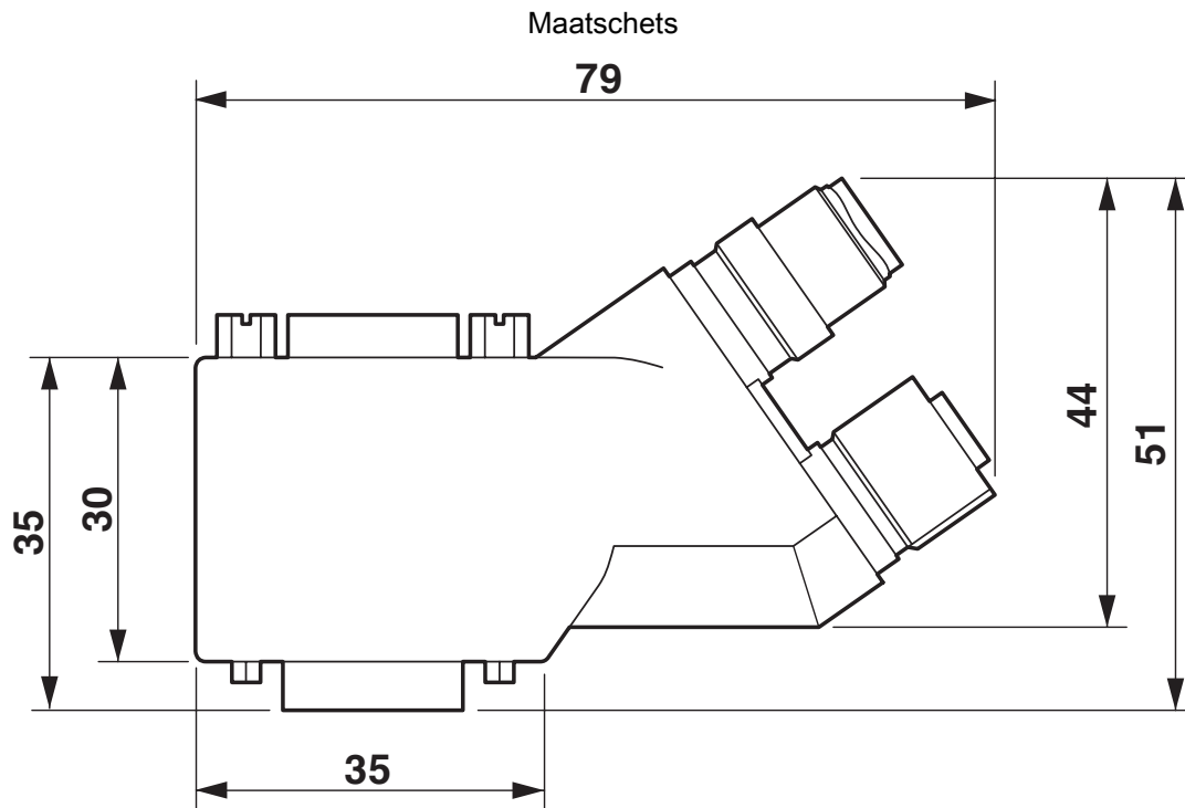
Maatschets SUBCON-PLUS...35...M12, 35°-variant
