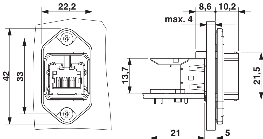
Push-pull-aanbouwraam, RJ45
