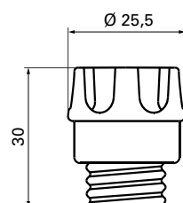
Fuse carrier/cap
