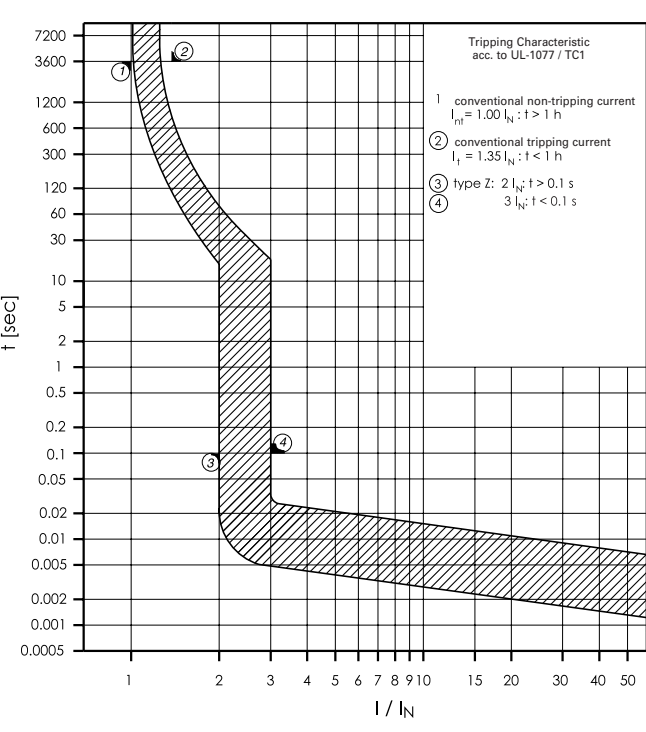
Characteristic Z - UL1077
