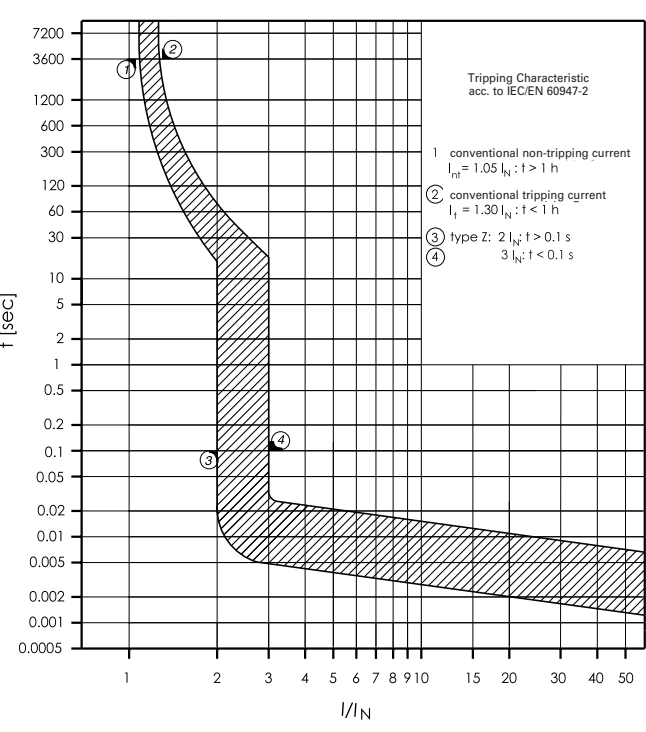
Characteristic Z - IEC/EN 60947-2
