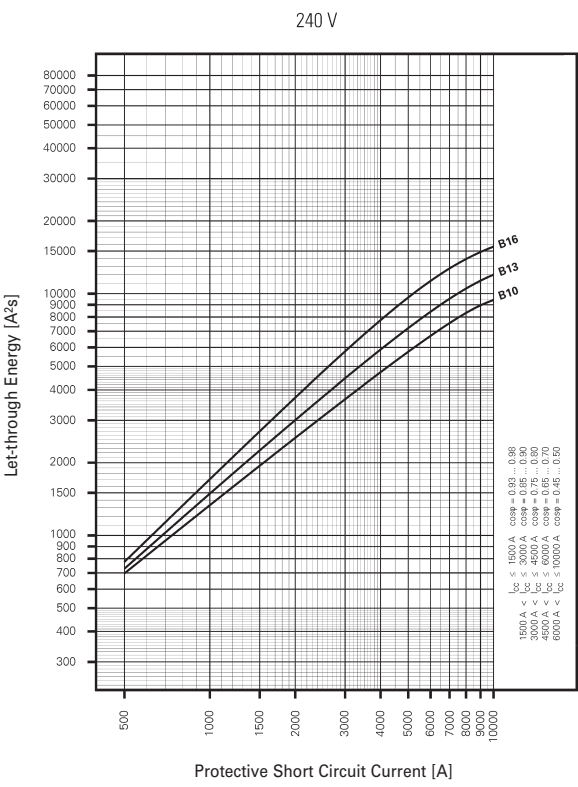
Let-through Energy FRBdM, Characteristic B
