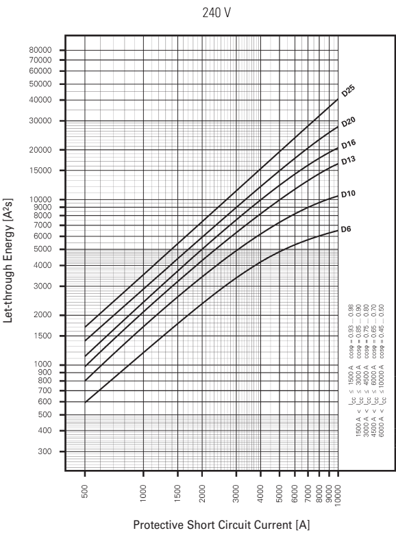
Let-through Energy FRBdM, Characteristic D
