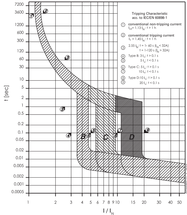
Characteristics B, C and D - EN60898
