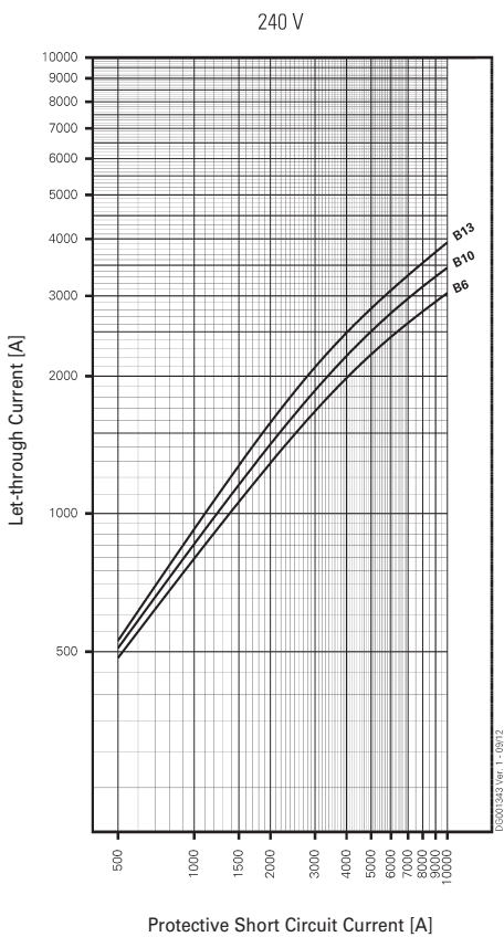
Let-through Current FRBdM, Characteristic B
