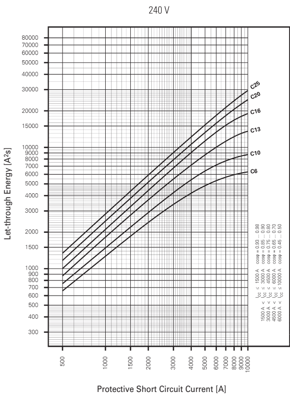
Let-through Energy FRBdM, Characteristic C
