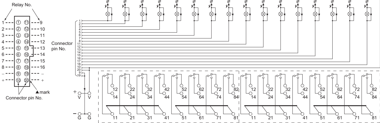
Connector Pin (male) Configuration View from engaged side
