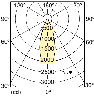
LDLD_CDM-Rm_20W_40D_0003-Light distribution diagram
