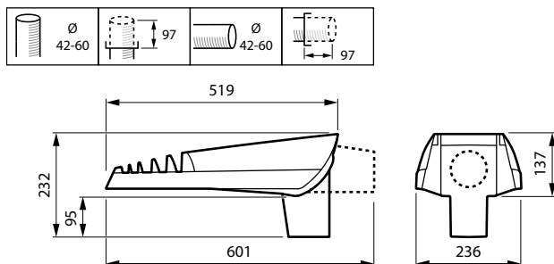
BGP701 LED40-4S/740 DM10 GF SRT SRB 42/6
