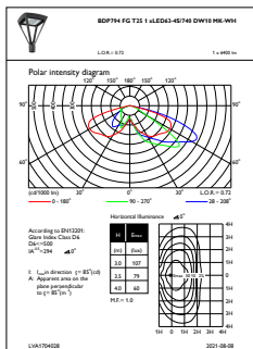
OFPL1_BDP794FGT251xLED63-4S740DW10MK-WH
