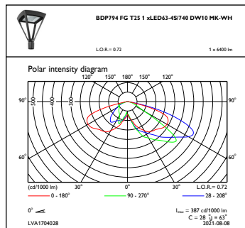
OFPC1_BDP794FGT251xLED63-4S740DW10MK-WH
