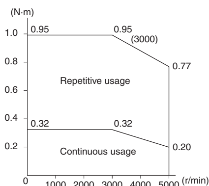
R88M-G10030L
