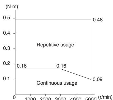
R88M-G05030H
