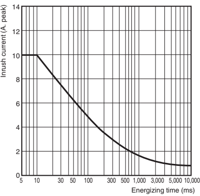
G3RZ-201SLN
