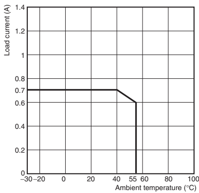
G3RZ-201SLN
