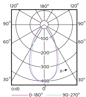
Light Distribution Diagram - MAS LED spot VLE D 4.9-50W GU10 927 60D
