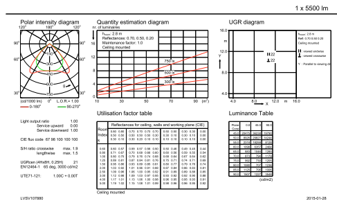
IFGU_4MX400 G3 491 1xLED55S/840 PSD WB-General uniform lighting
