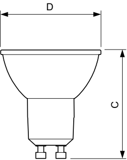
GU10 230V 4W-35W 260lm 60D 2700K GU10 ND
